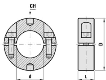
AM/SA (separable clamping ring)
